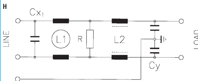
Circuit diagram
