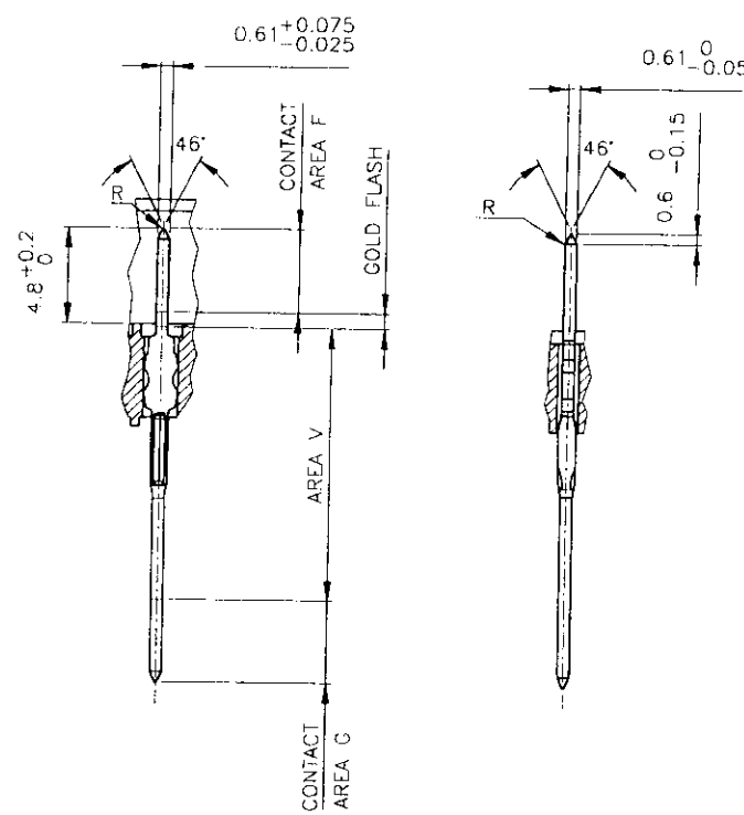
DETAIL P SCALE 5:1
