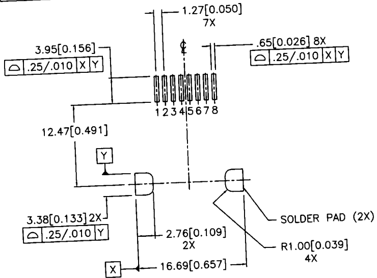
RECOMMENDED P.C.B. LAYOUT AS VIEWED FROM TOP SIDE (COMPONENT SIDE)
