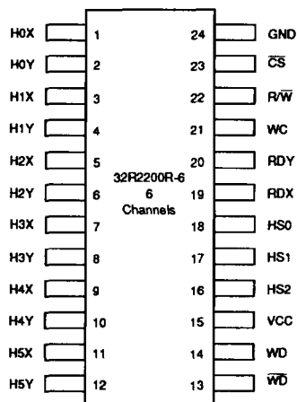
24-Lead SOV, SOL
