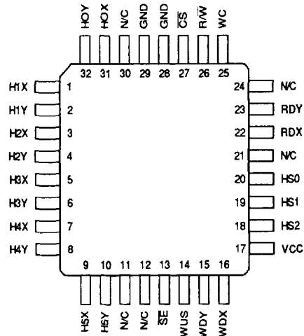
6-Channel 32-Lead TQFP
