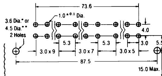
For 48 Circuit
