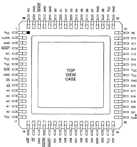
Figure 2.2. : CQFP terminal designation.
