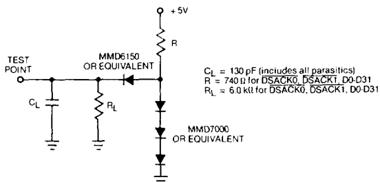
Figure 5 : Test loads.
