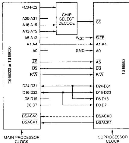
Figure 19 : 16-bit data bus coprocessor connection.
