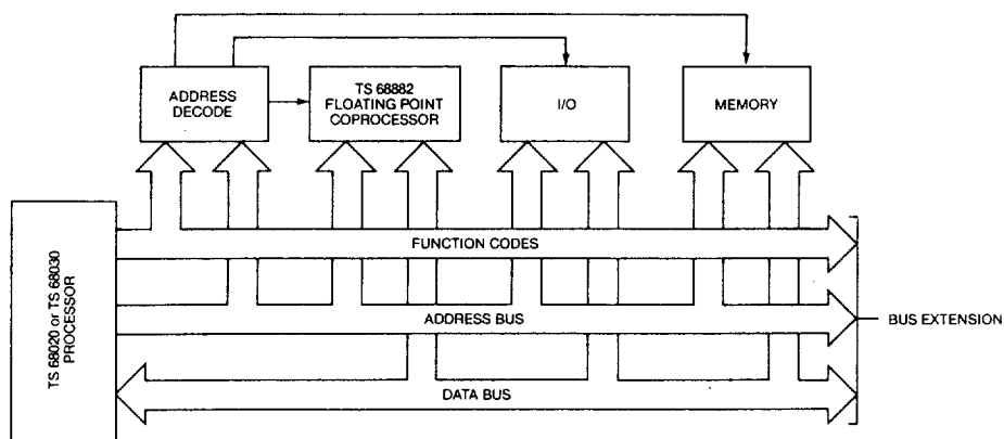
Figure 16 : Typical coprocessor configuration.
