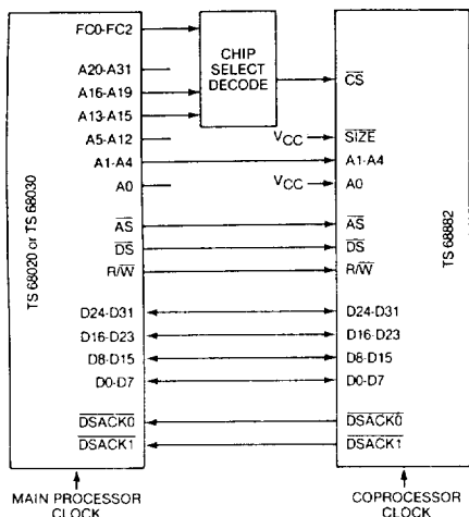
Figure 18 : 32-bit data bus coprocessor connection.
