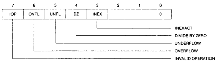
Figure 15 : Accrued exception byte.
