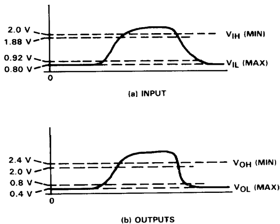
FIGURE 4. VOLTAGE REFERENCE LEVELS
