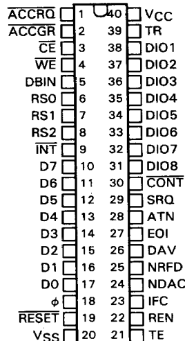
JD PACKAGE (TOP VIEW)
