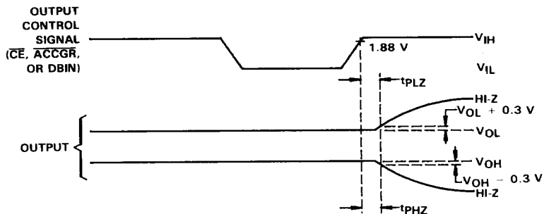
FIGURE 5. HIGH-IMPEDANCE MEASUREMENTS
