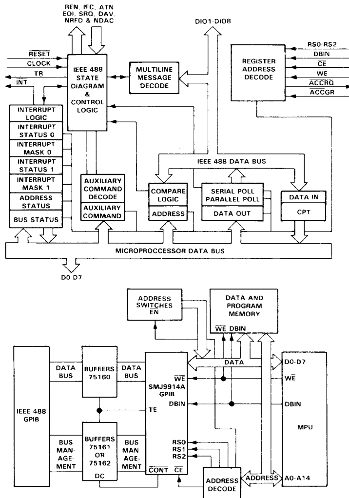
FIGURE 1. TYPICAL SMJ9914A APPLICATION
