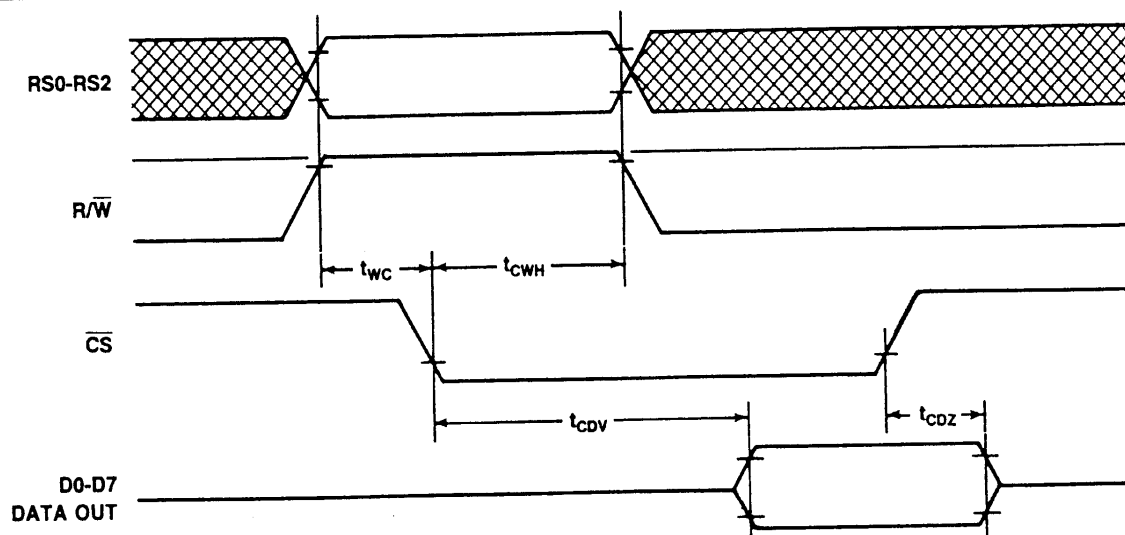
DACIA Read Cycle Waveforms
