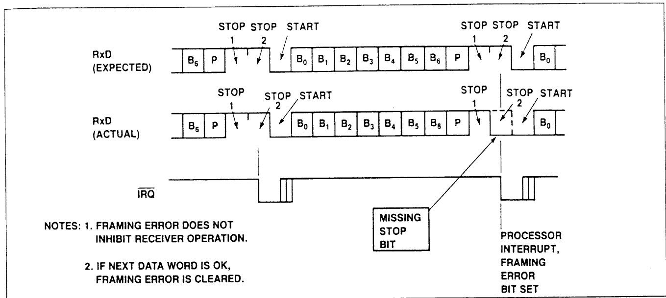
Figure 12. Framing Error
