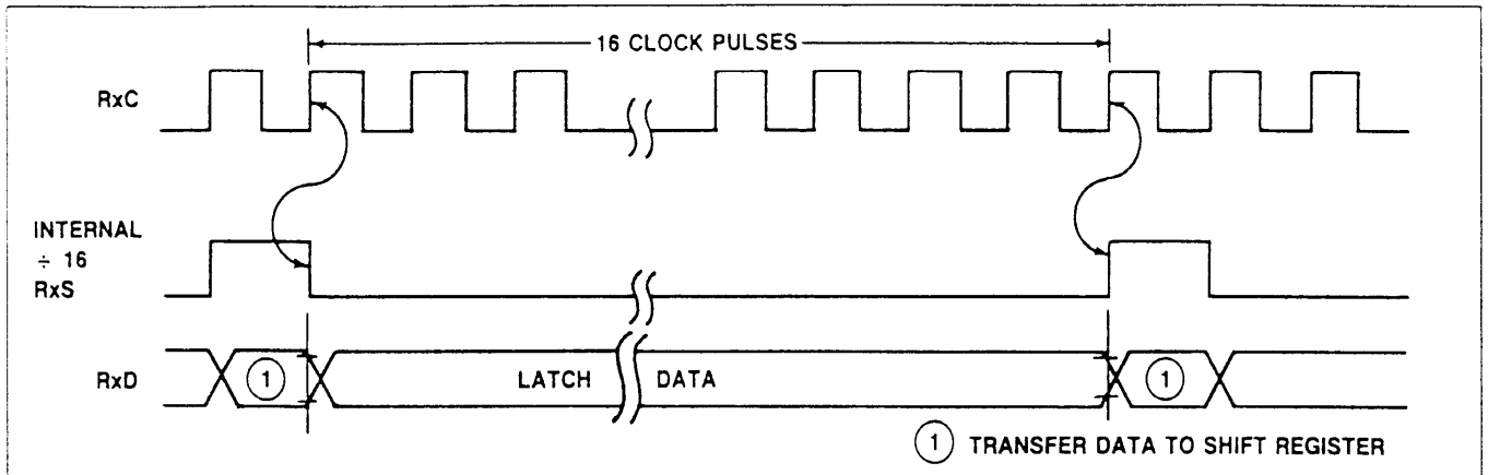
Figure 15. DACIA External Clock Timing — Receive Data
