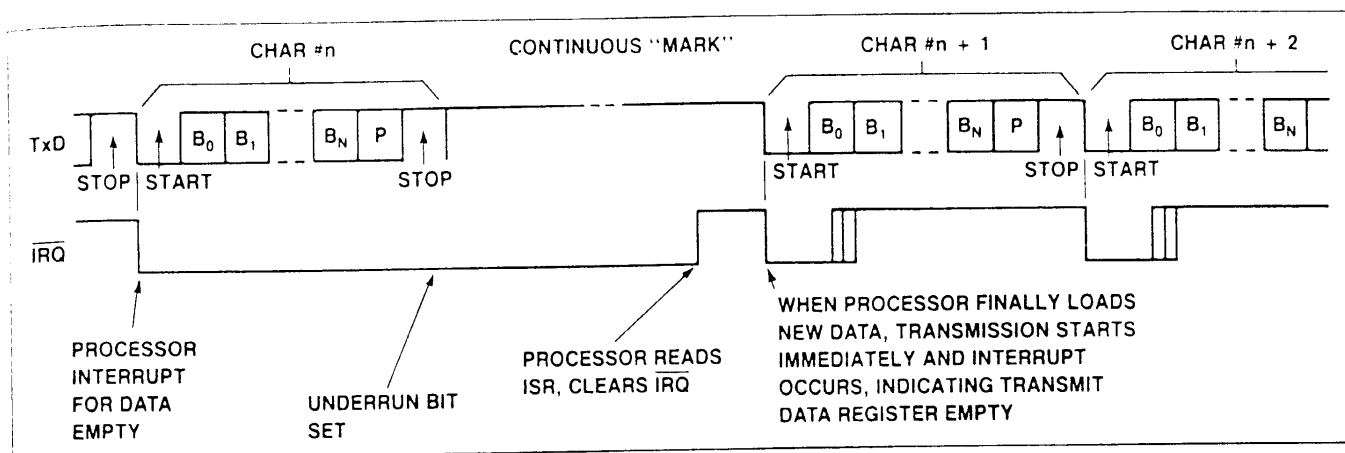
Figure 8. Transmit Underrun Condition Relationship
