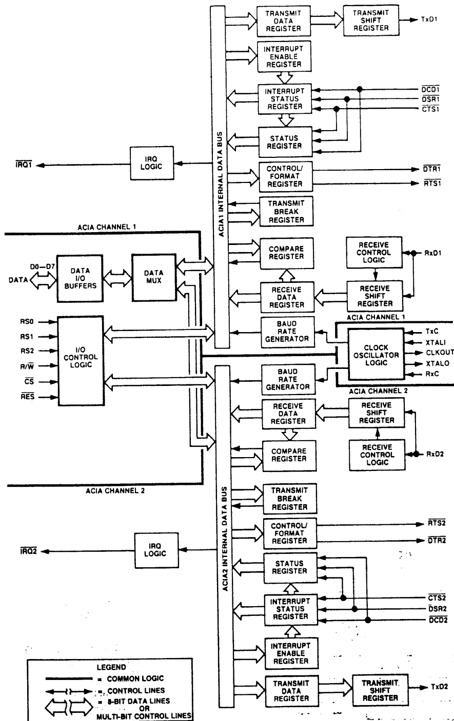
Figure 3. DACIA Block Diagram
