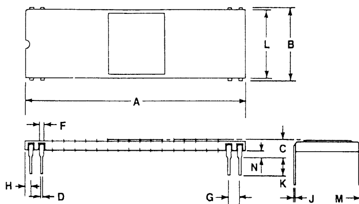
40-PIN CERAMIC DIP
