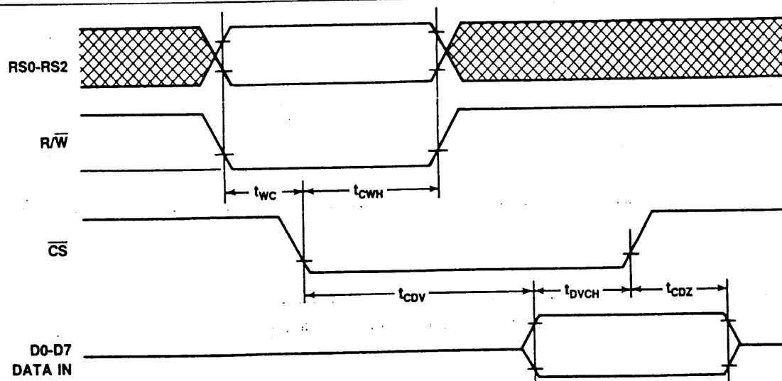
DACIA Write Cycle Waveforms
