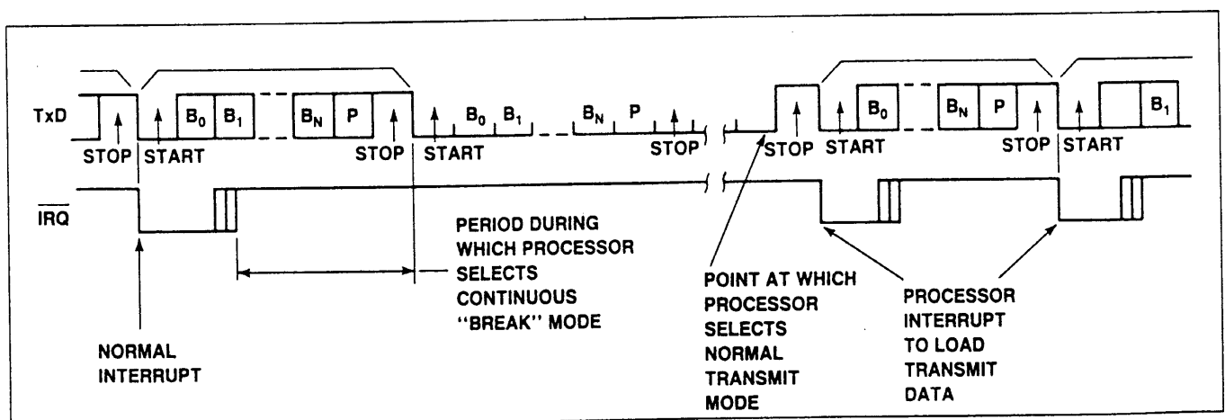
Figure 13. Transmit Break Character
