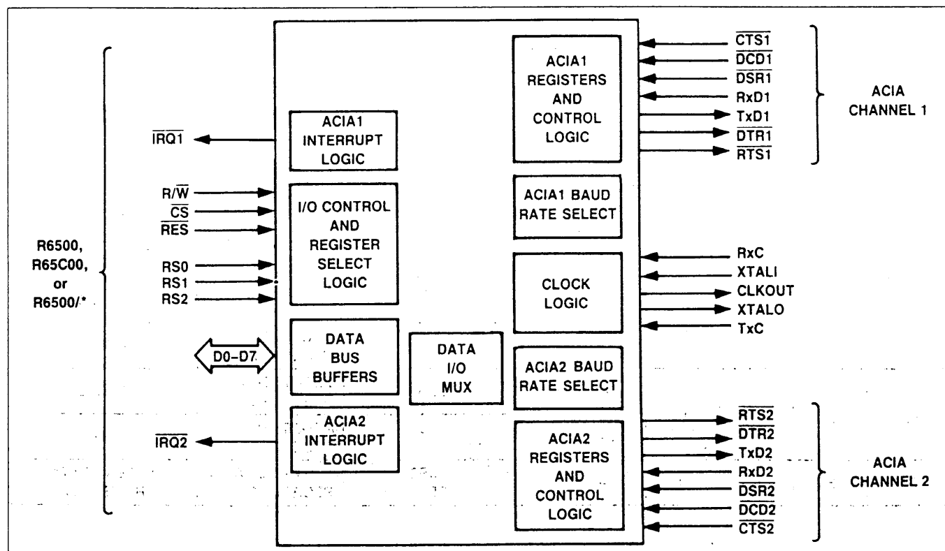
Figure 2. DACIA Interface Signals
