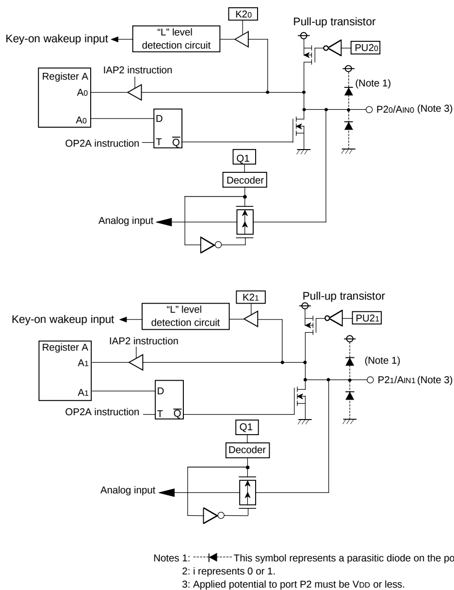
Port block diagram (4)
