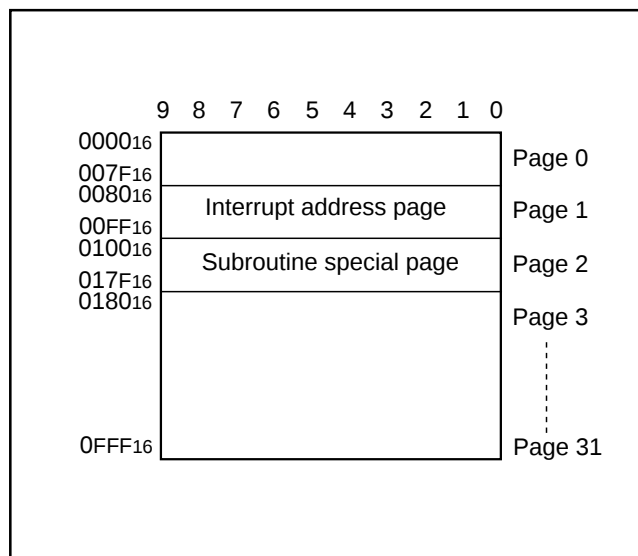
Fig. 10 ROM map of M34506M4/M34506E4
