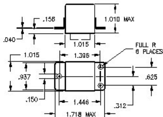
MOUNTING STYLE D (USE SO-1057-8912)
