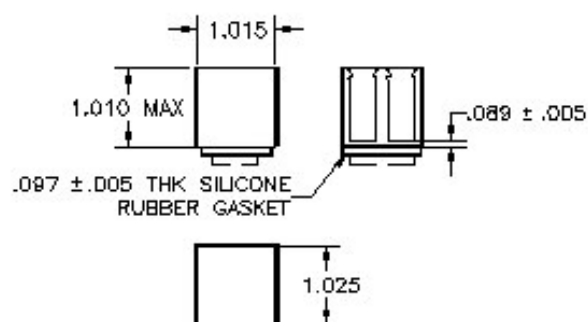
MOUNTING STYLE W
