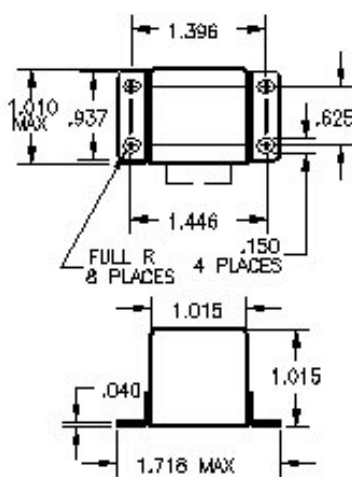
MOUNTING STYLE J
