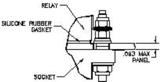
HARDWARE MOUNTING MOUNTING DETAIL 4 PLACES
