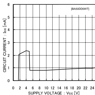
Fig.13 Circuit Current
