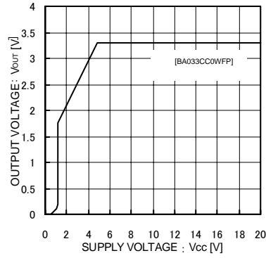
Fig.2 Input Stability
