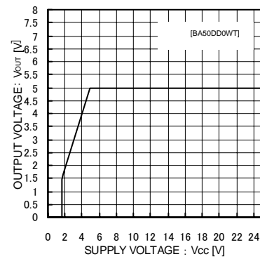
Fig.15 Input Stability
