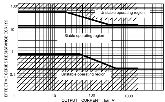
Fig.34 ESR vs I_o Characteristics (BA□□DD0,22 \mu\text{F} )
