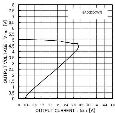
Fig.16 Load Stability
