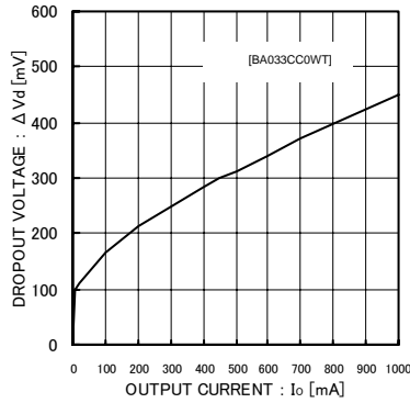
Fig.5 Input/Output Voltage Difference ( I_{OUT}=0V \rightarrow 1A )
