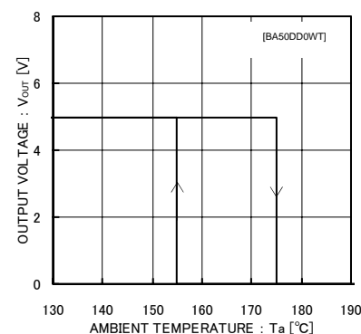
Fig.24 Thermal Shutdown
