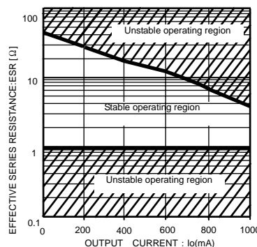
Fig.33 ESR- I_o Characteristics (BA□□CC0,22 \mu\text{F} )
