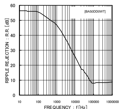
Fig.18 Ripple Rejection Characteristics ( I_{out}=100mA )
