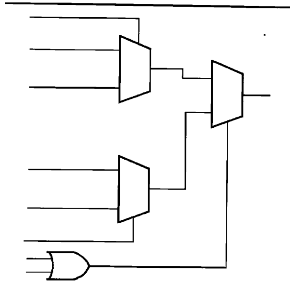
Figure 1 • 40MX Logic Module
