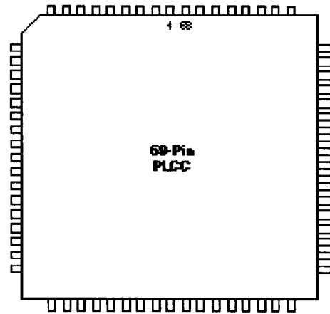
68-Pin PLCC
