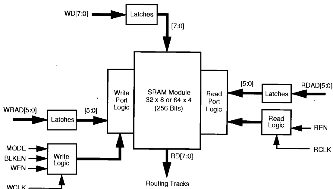
Figure 5• 42MX Dual-Port SRAM Block
