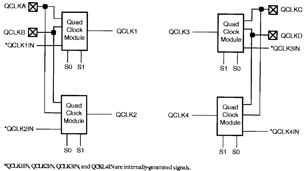
Figure 9• Quadrant Clock Network
