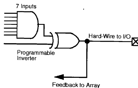
Figure 4• D-Module Implementation
