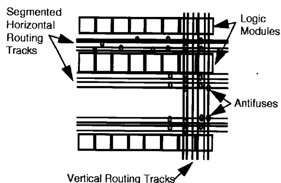
Figure 7• Routing Structure
