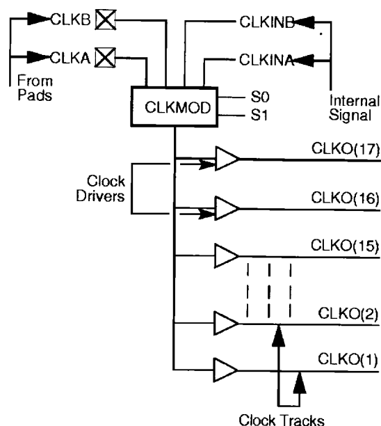
Figure 8• Clock Networks
