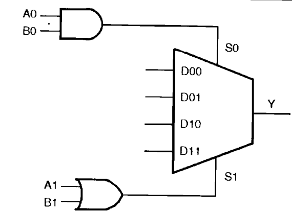
Figure 2• C-Module Implementation
