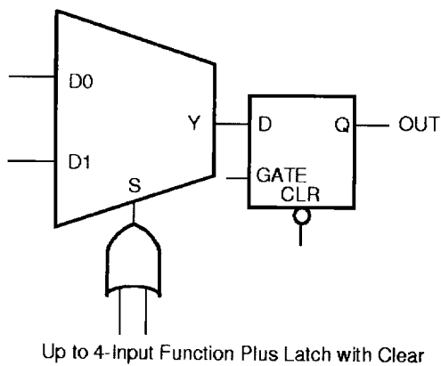
Figure 3• S-Module Implementation
