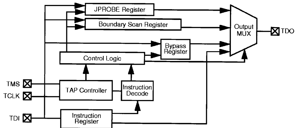
Figure 10• JTAG BST Circuitry
