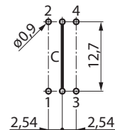
Drilling diagram (View from mounting side)
