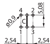
Drilling diagram (View from mounting side)
