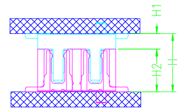
ASSEMBLY
