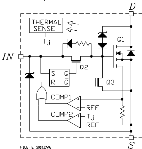
Fig.20 Block Diagram
