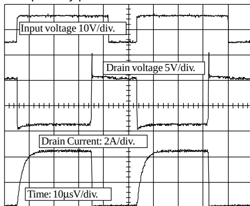
Fig. 24 Over-temperature shut-down
