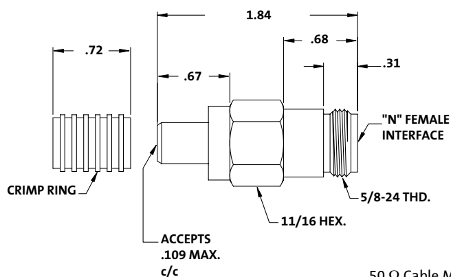
50 Ω Cable Mount Female N
