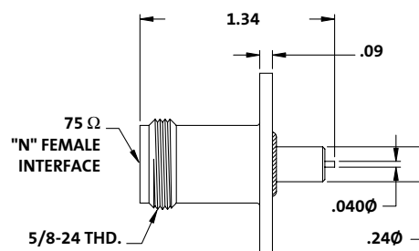
75 Ω Bulkhead Mount N
