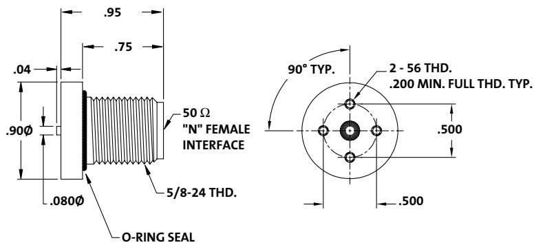
50 Ω N PCB Four Hole Mount
