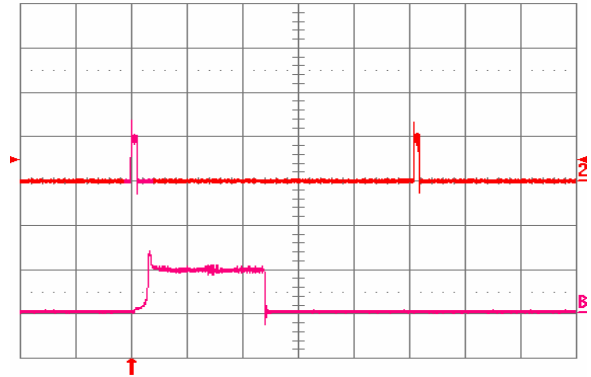
Fig. 2.5V.18: Load current (top trace, 20 A/div., 20 ms/div.) into a 10 mΩ short circuit during restart, at V in = 24V. Bottom trace (20 A/div., 1 ms/div.) is an expansion of the on-time portion of the top trace.
