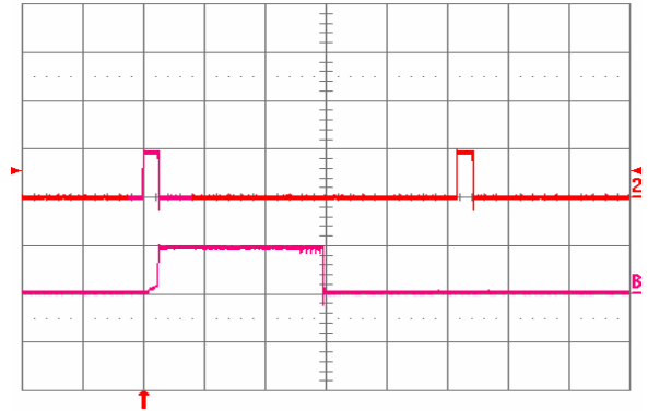
Fig. 1.2V.18: Load current (top trace, 20 A/div., 20 ms/div.) into a 10 mΩ short circuit during restart, at V in = 24V. Bottom trace (20 A/div., 2 ms/div.) is an expansion of the on-time portion of the top trace.
