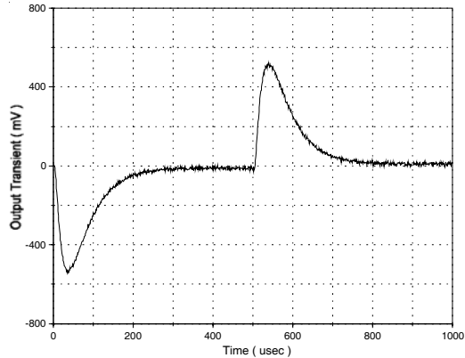
Fig.34 Output Load Transient Response 50% Load to/from 100% Load
