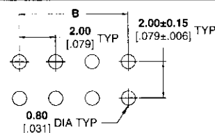
Recommended Solder Pad Layout
