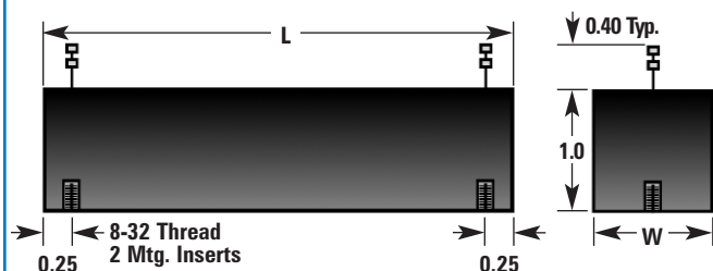
Figure 11-Rectifier Block
