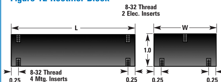
Figure 12-Rectifier Block
