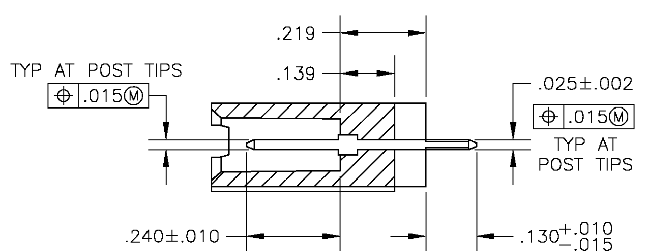
SECTION X—X
