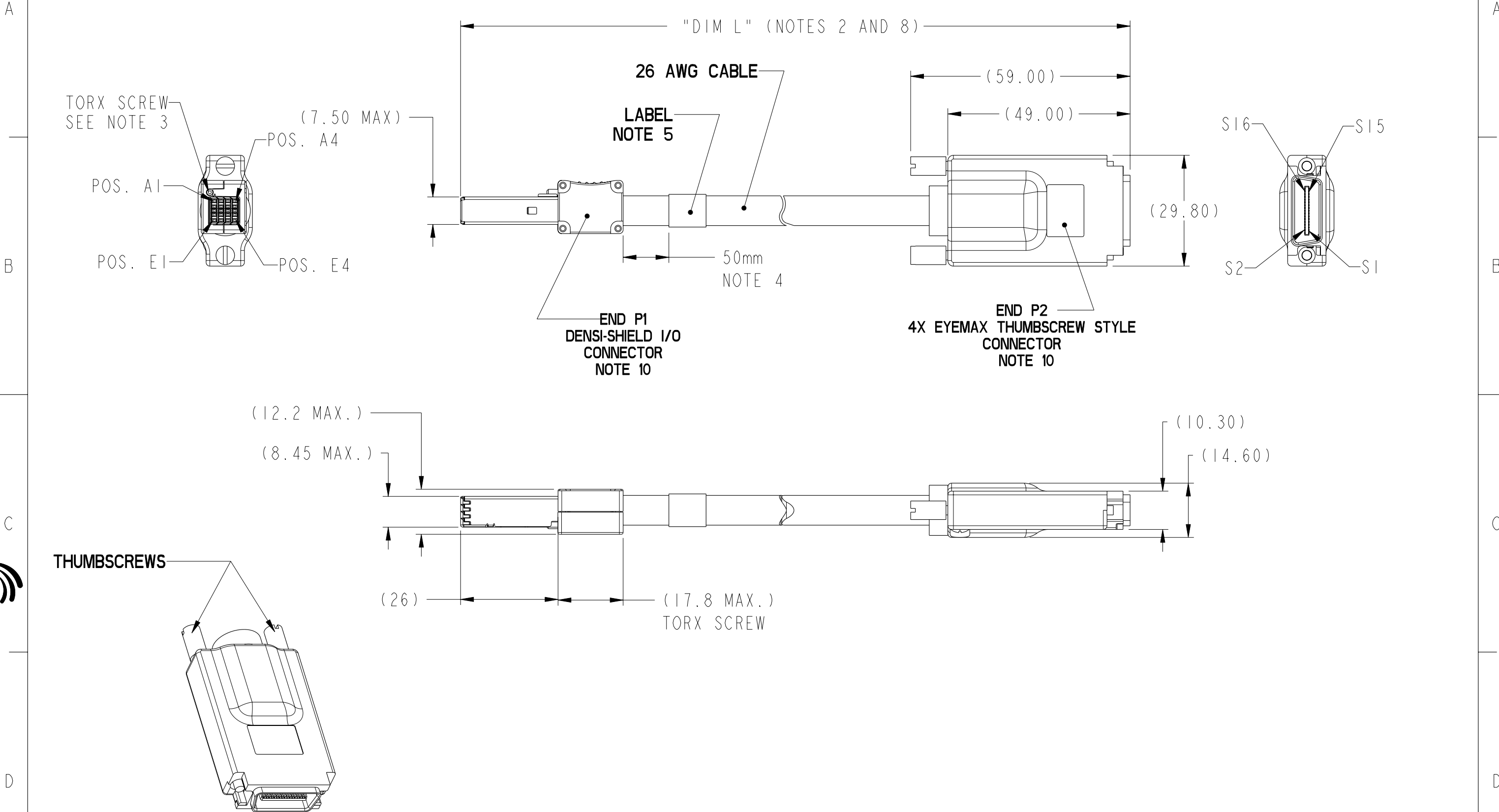
EYEMAX - THUMBSCREW STYLE ISOMETRIC VIEW
