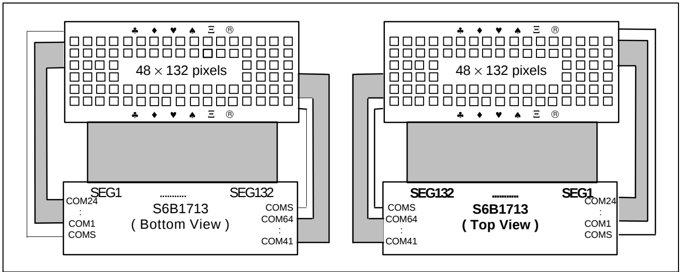
Figure 46. SHL = 0, ADC = 0 Figure 47. SHL = 0, ADC = 1
