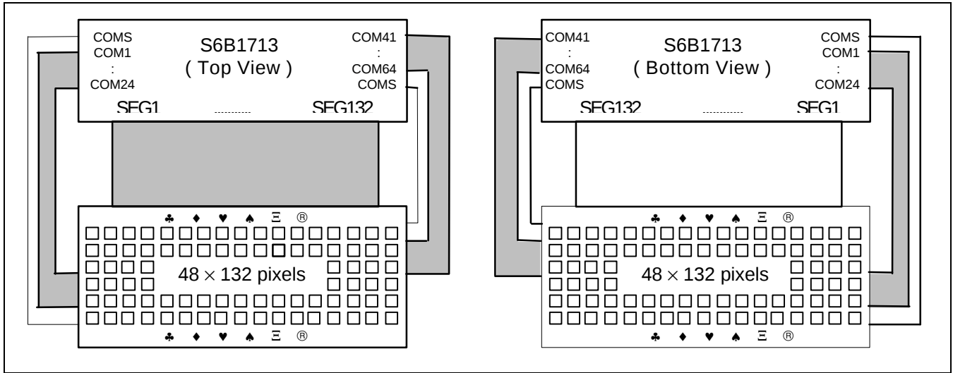
Figure 48. SHL = 1, ADC = 0 Figure 49. SHL = 1, ADC = 1
