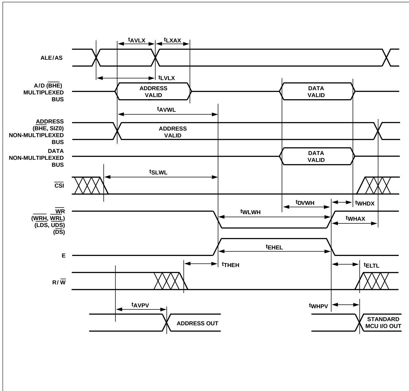
Figure 40. Write Timing
