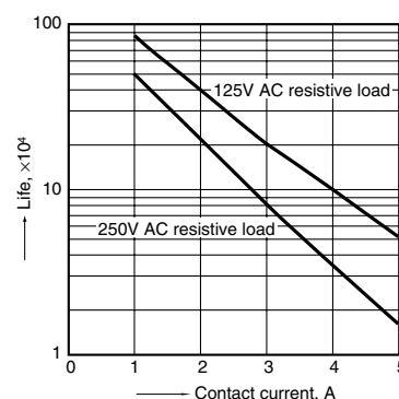
2. Life curve
