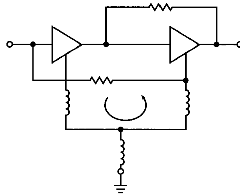
Figure 1. INA Potential Ground Loop
