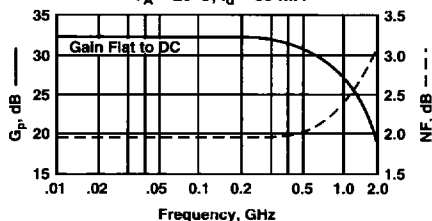
Typical Gain and Noise Figure vs. Frequency T_A = 25^\circ\text{C} , I_d = 35\text{ mA}
