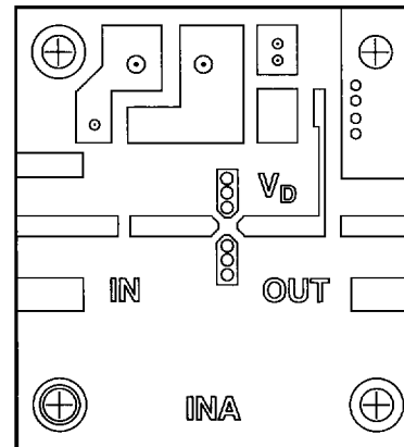
Figure 2. INA Circuit Board 2x Actual Size
