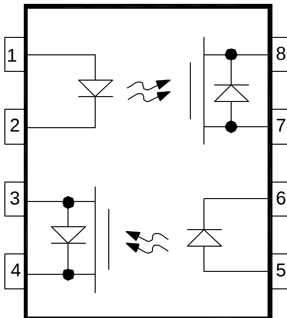
FIGURE 2. Terminal connections.
