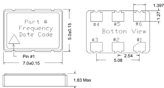
Figure 4. VCC6-QCx and VCC6-QAx Package Drawing
