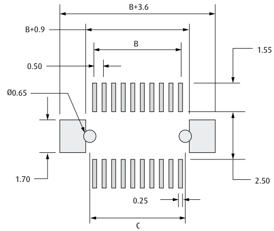
Recommended PC Board Pattern
