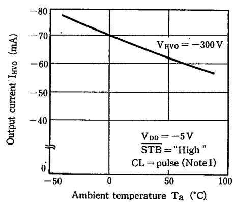
Output current vs. Ambient temperature
