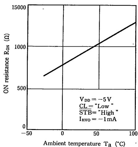
ON resistance vs. Ambient temperature
