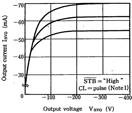
Output current vs. Output voltage
