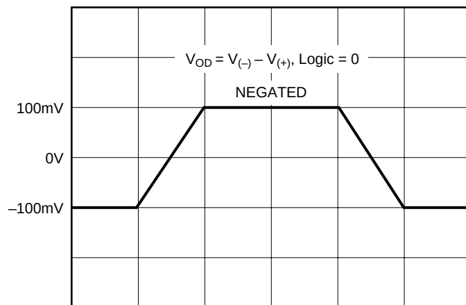
Figure 2. V_{OD}
