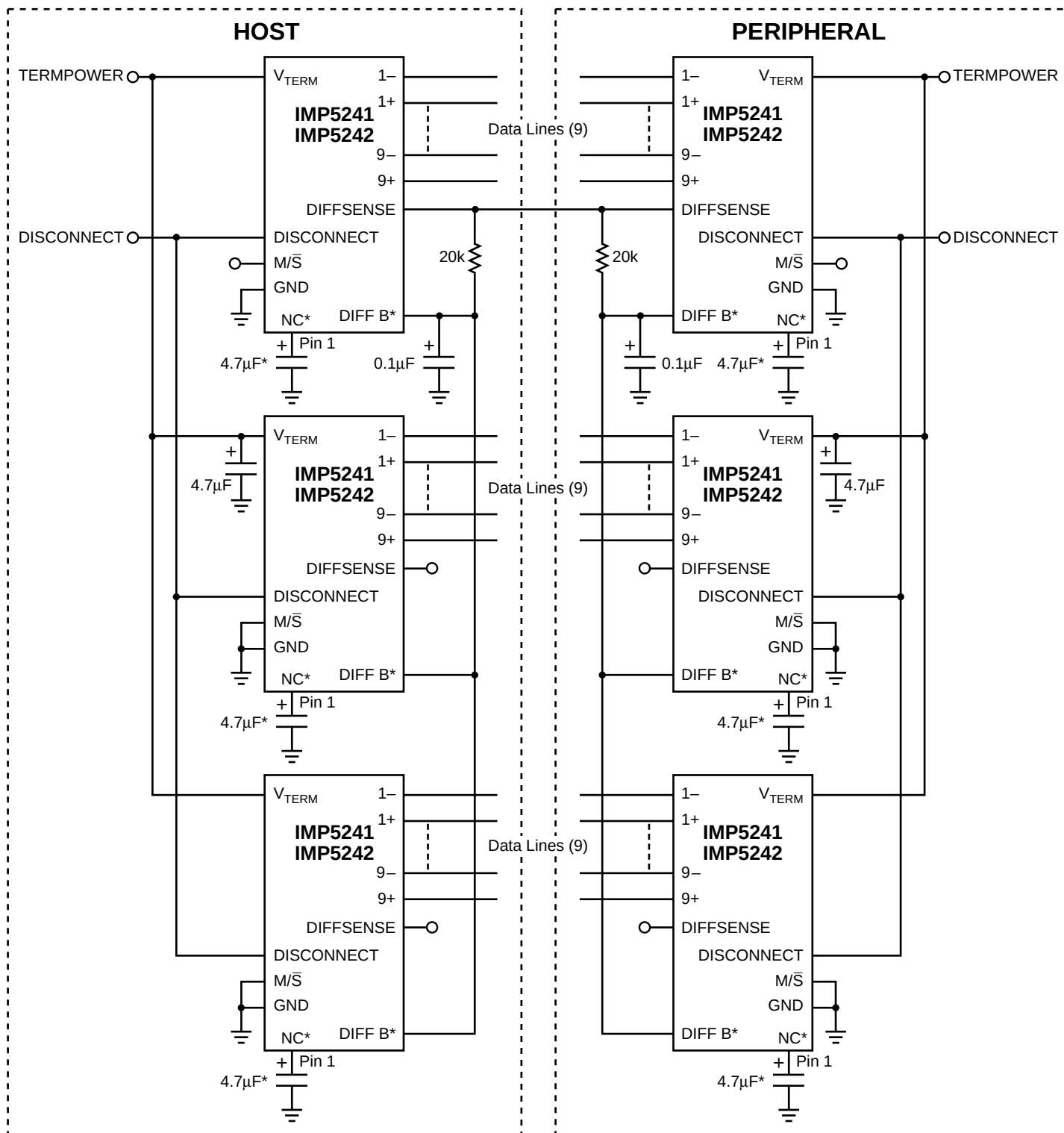
Figure 5. Suggested IMP5241/5242 Universal Application Schematic (Please reference manufacture's current data sheet to ensure compatibility)
