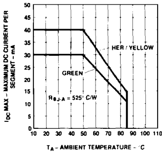
Figure 9. Maximum Allowable DC Current vs. Ambient Temperature.
