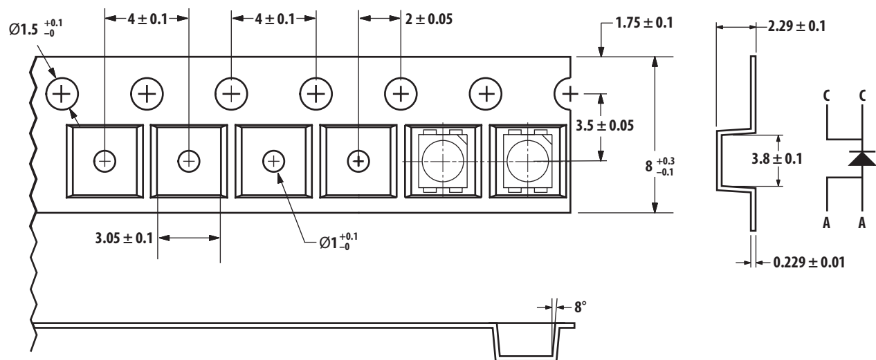
Figure 15. Tape Dimensions
