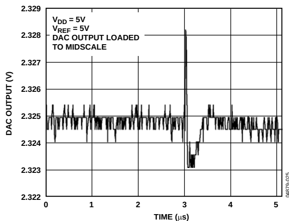
Figure 25. DAC-to-DAC Crosstalk
