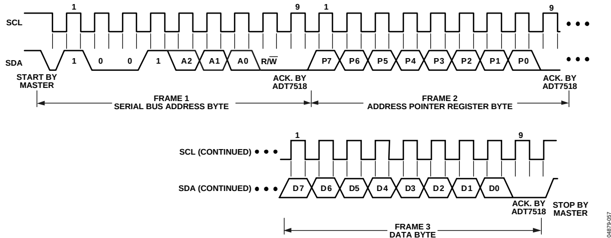
Figure 57. I 2 C—Writing to the Address Pointer Register Followed by a Single Byte of Data to the Selected Register
