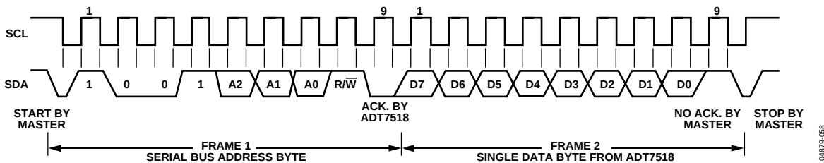
Figure 58. I 2 C—Reading a Single Byte of Data from a Selected Register
