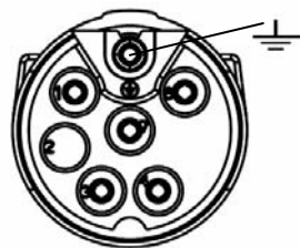
connector view to the mating side
