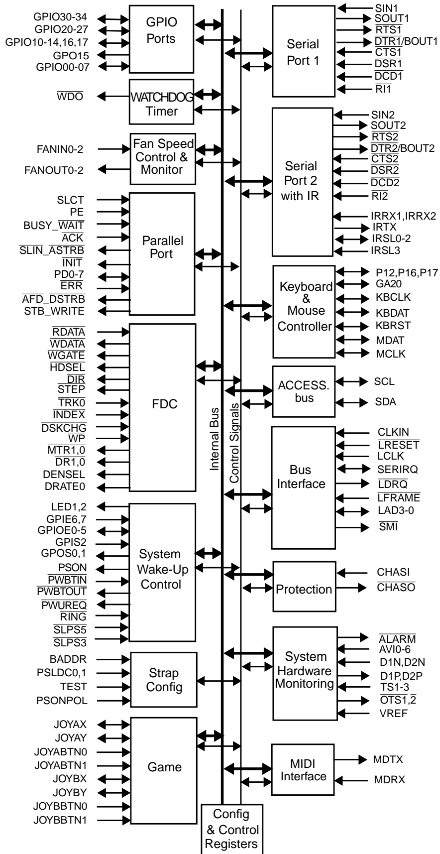
Figure 1. PC87366 Detailed Block Diagram
