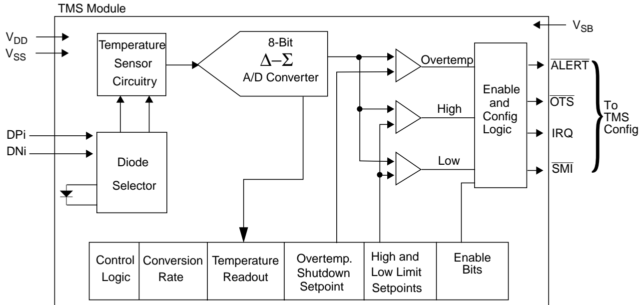
Figure 41. TMS Simplified Block Diagram
