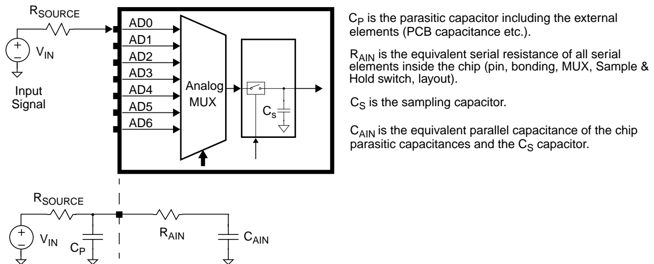
Figure 39. Analog Input Schematic Diagram and Equivalent R-C Circuit
