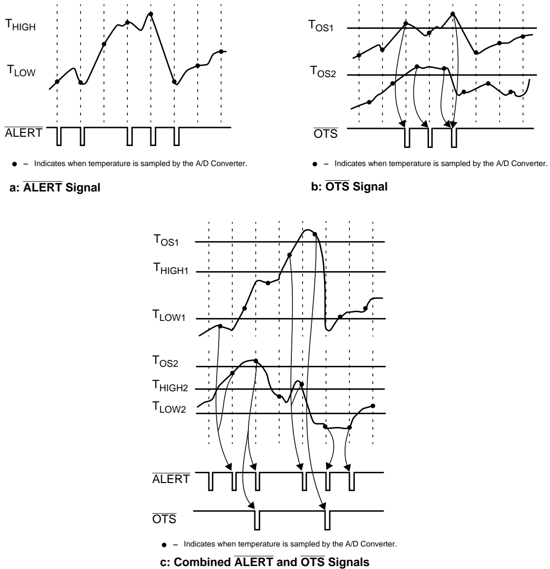
Figure 43. OTS and ALERT Temperature Response Diagrams
