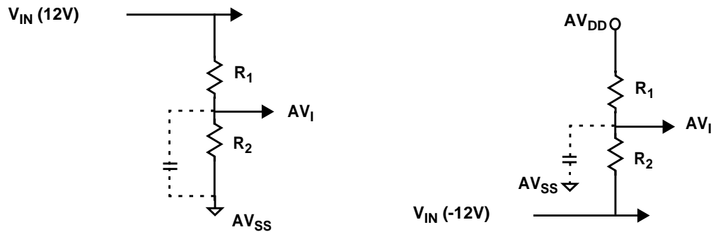
Figure 40. Measurement Out of Positive and Negative Voltages
