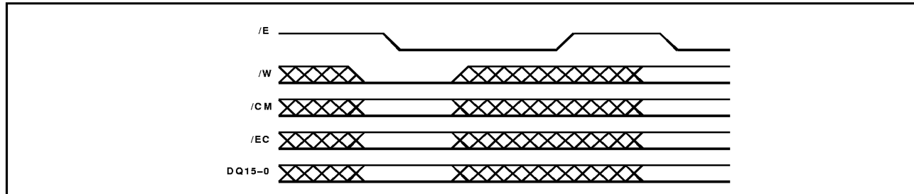
Figure 4: Write Cycle
