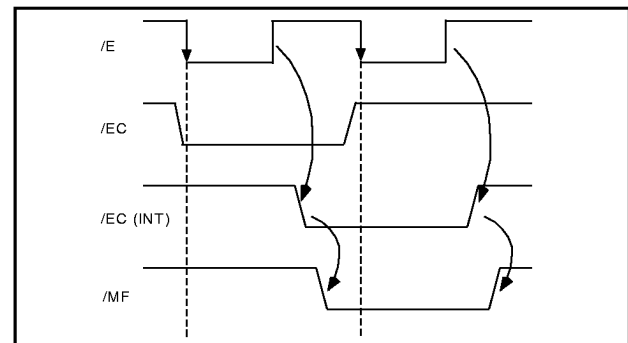
Figure 6: /EC(Int) Timing Diagram
