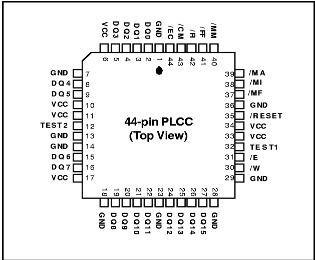
PINOUT DIAGRAM
