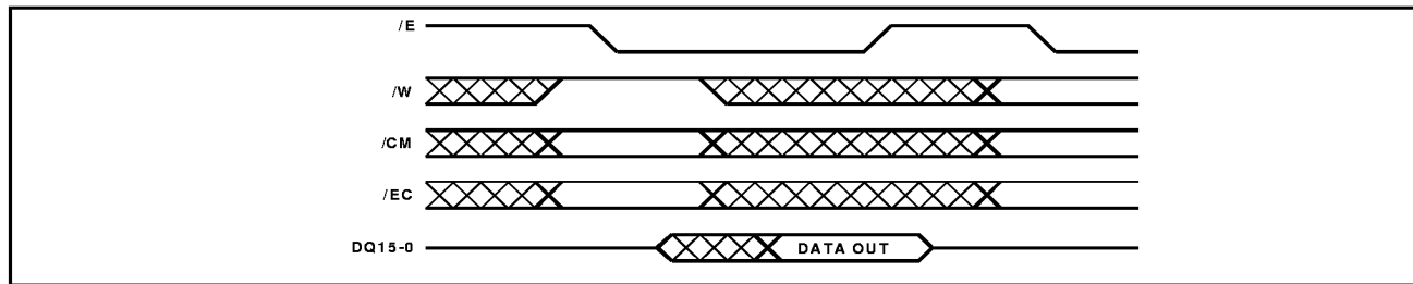
Figure 3: Read Cycle
