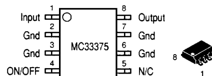
D SUFFIX PLASTIC PACKAGE CASE 751-06 (SOP-8)
