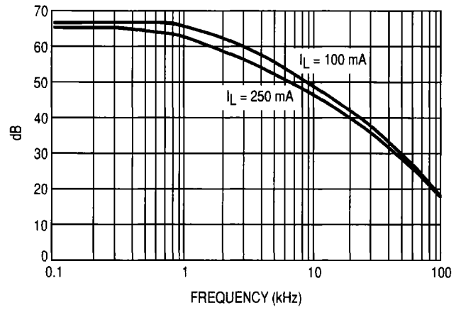
Figure 13. Ripple Rejection
