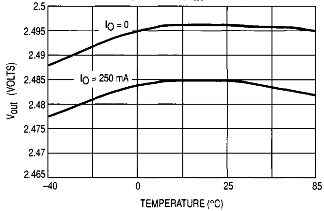
Figure 11. Output Voltage versus Ambient Temperature ( V_{in} = 12\text{ V} )
