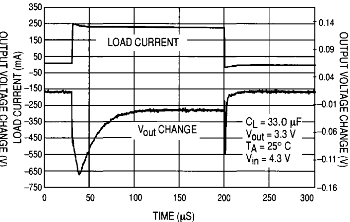
Figure 4. Load Transient Response
