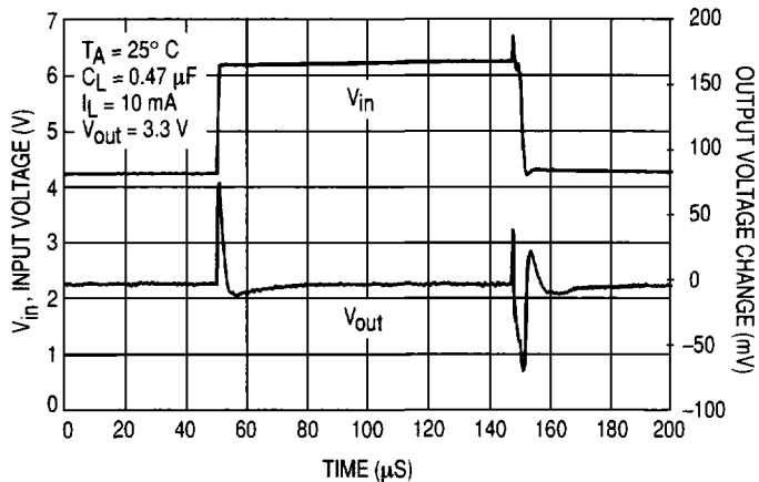
Figure 1. Line Transient Response
