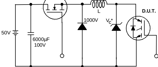
Figure 19. Clamped Inductive Load Test Circuit
