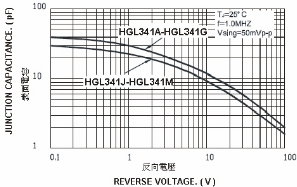
FIG. 5 – 表面電容(典型值) FIG. 5 – TYPICAL JUNCTION CAPACITANCE
