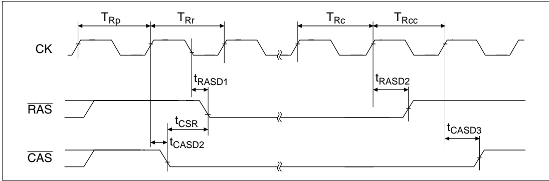
Figure 20.18 Self-Refresh
