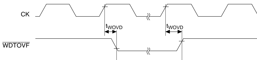
Figure 20.39 Watchdog Timer Output Timing
