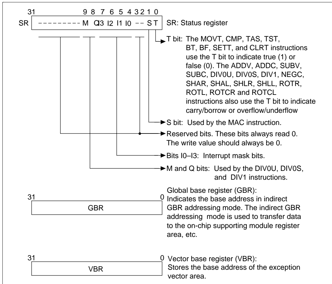
Figure 2.2 Control Registers
