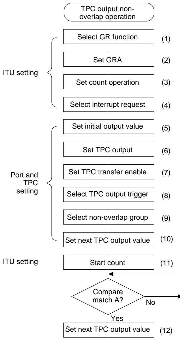
Figure 11.6 Example of Setting Procedure for TPC Output Non-Overlap Operation
