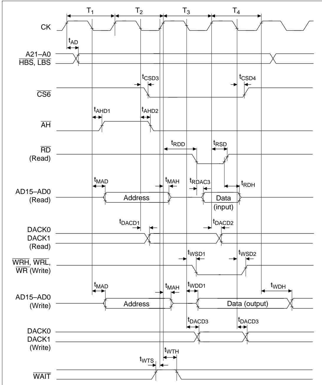
Figure 20.19 Address/Data Multiplex I/O Bus Cycle
