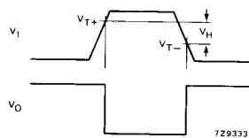
Fig. 7 Waveforms showing the definition of V_{T+} , V_{T-} and V_H .
