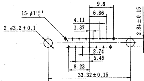
SDAB-15
