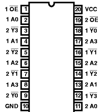
20 LEAD CERAMIC METAL SEAL FLATPACK PACKAGE (FLATPACK) MIL-STD-1835 CDFP4-F20, LEAD FINISH C TOP VIEW
