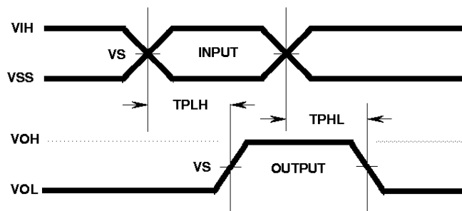
VOLTAGE LEVELS
