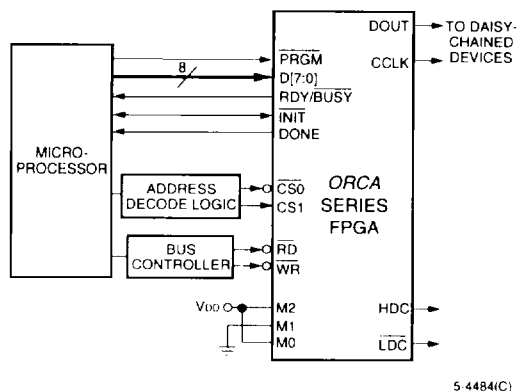
Figure 43. Asynchronous Peripheral Configuration Schematic
