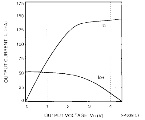
Figure 83. Fast ( T_j = 125^\circ\text{C} , V_{DD} = 4.5\text{ V} )
