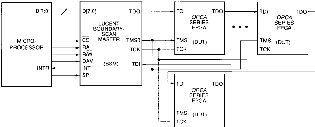
Figure 49. Boundary-Scan Interface
