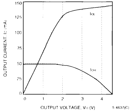
Figure 82. Slewlim ( T_j = 125^\circ\text{C} , V_{DD} = 4.5\text{ V} )
