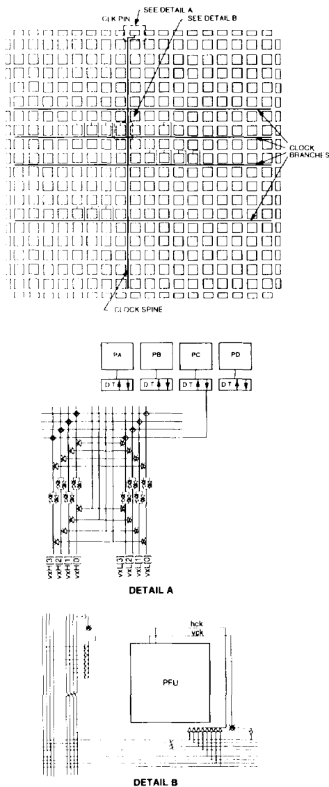
Figure 35. Secondary Clock Distribution
