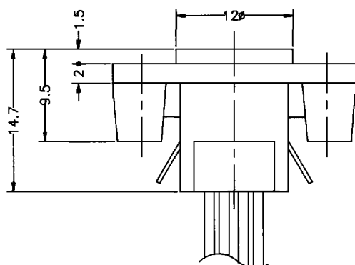
WITHOUT SHIELD
