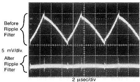
FIGURE 17. Post Ripple Filter Waveform
