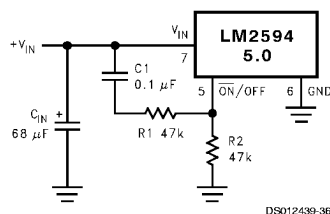
FIGURE 21. Delayed Startup
