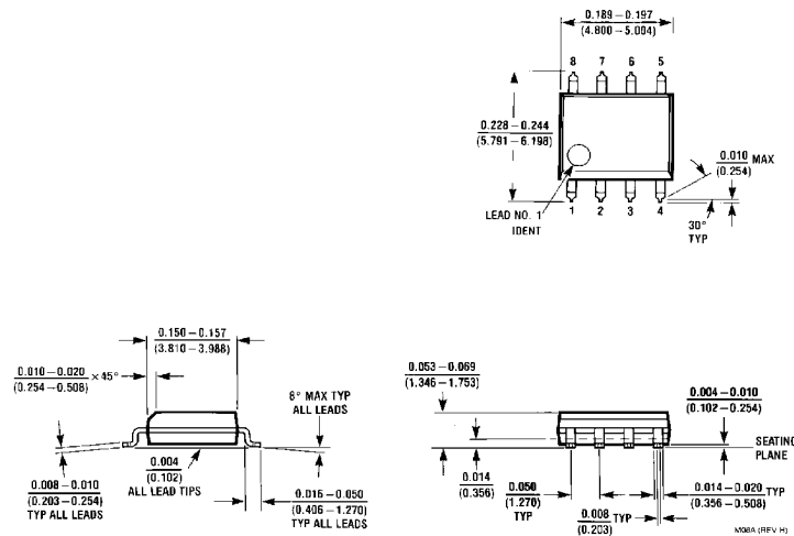
8-Lead (0.150" Wide) Molded Small Outline Package, Order Number LM2594M-3.3, LM2594M-5.0, LM2594M-12 or LM2594M-ADJ JEDEC NS Package Number M08A
