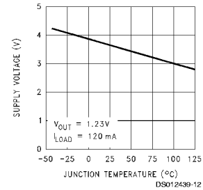
Minimum Operating Supply Voltage
