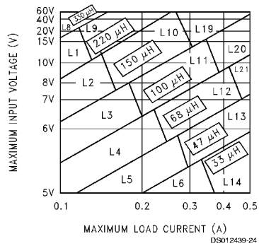
FIGURE 4. LM2594/LM2594HV-3.3
