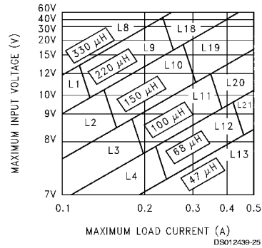
FIGURE 5. LM2594/LM2594HV-5.0
