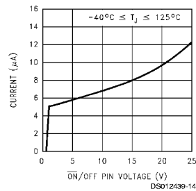
ON /OFF Pin Current (Sinking)
