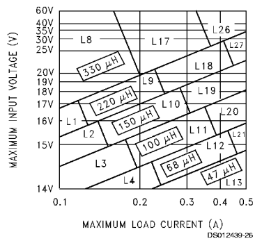
FIGURE 6. LM2594/LM2594HV-12
