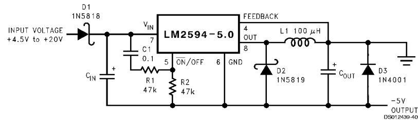
FIGURE 24. Undervoltage Lockout with Hysteresis for Inverting Regulator
