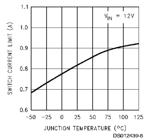
Switch Current Limit
