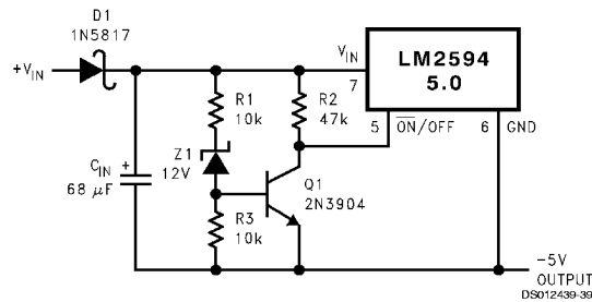
FIGURE 23. Undervoltage Lockout for Inverting Regulator
