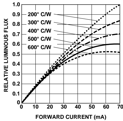
Figure 4. HPWT-xx00 Relative Luminous Flux vs. Forward Current.
