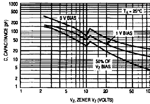
Figure 5. Typical Capacitance
