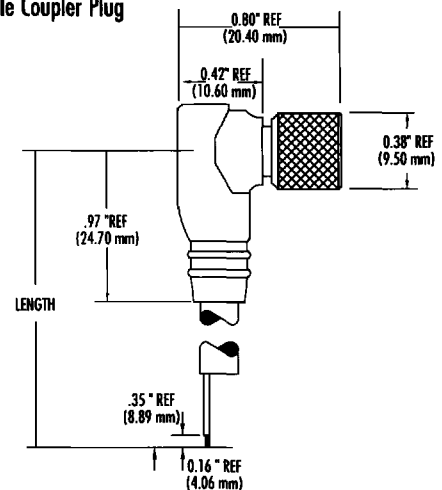
90° Female Coupler Plug
