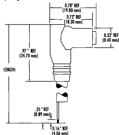
90° Female Snap Plug
